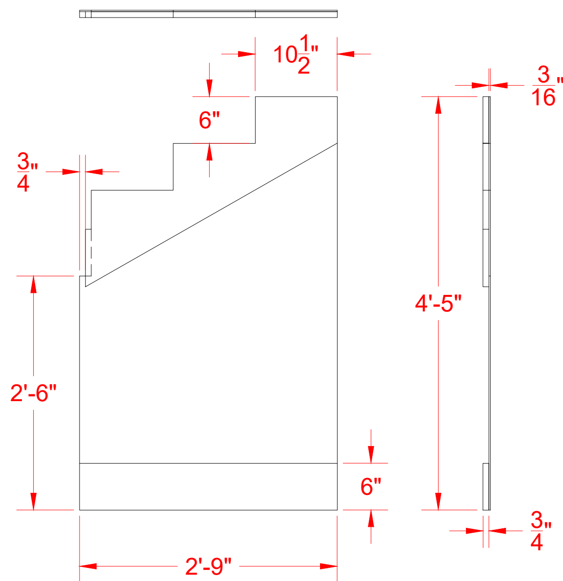
04 UPPER DETAIL FLAT 101 SCALE: 1"=1'-0"
