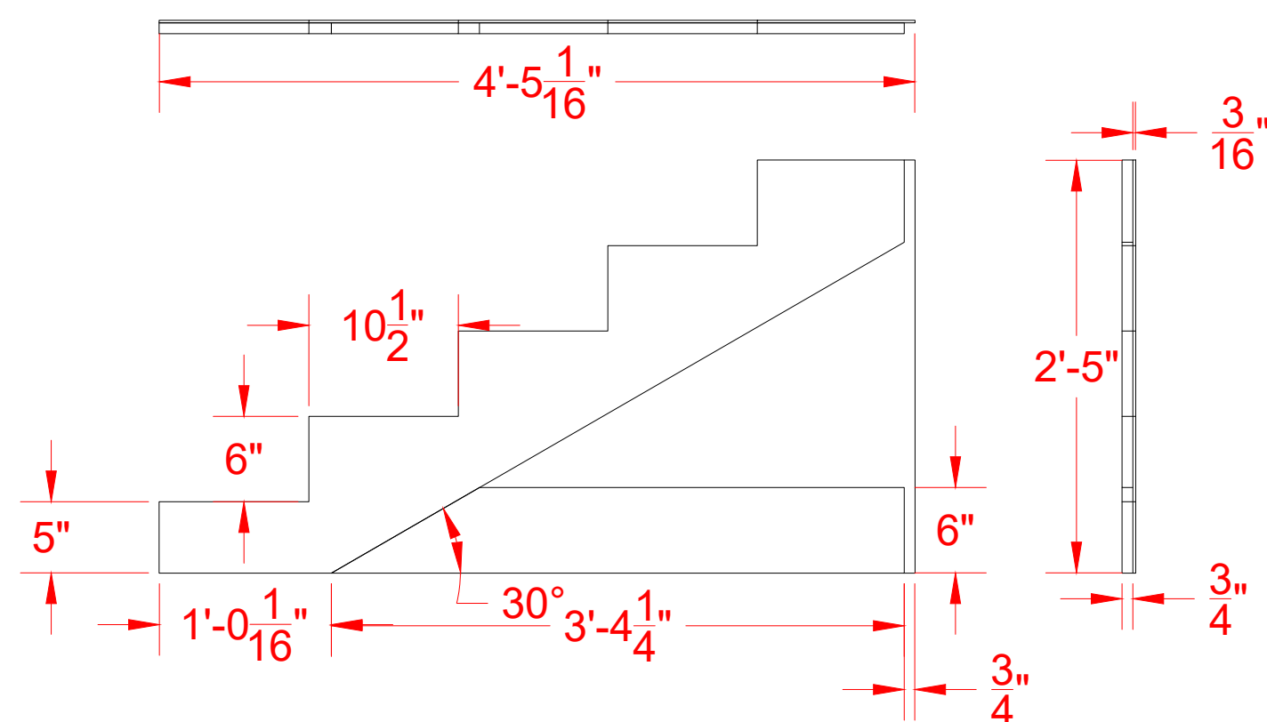
03 LOWER DETAIL FLAT 101 SCALE: 1"=1'-0"
