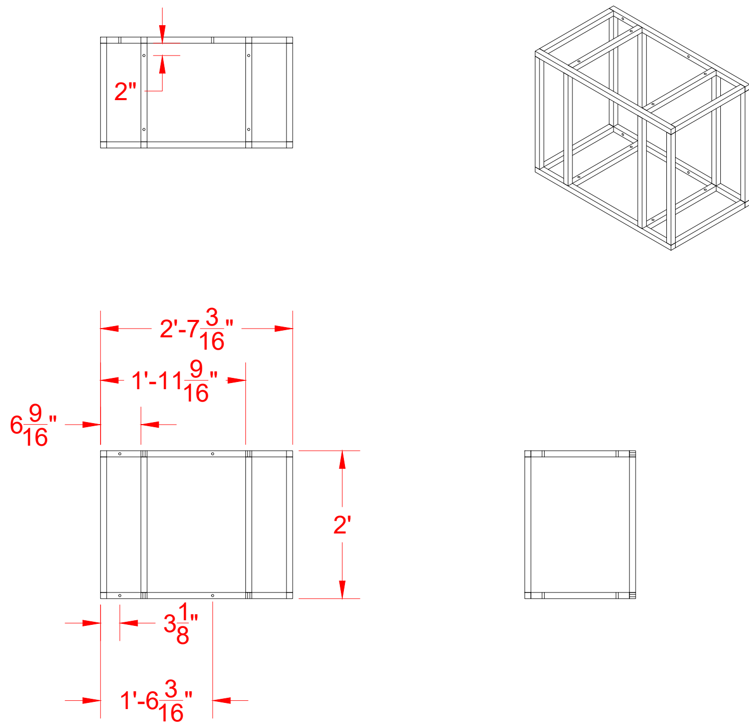
03 JUNCTION BLOCK 102 SCALE: 3/4" = 1'-0"
